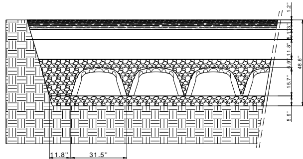
Fig. 1 – System cross-section
