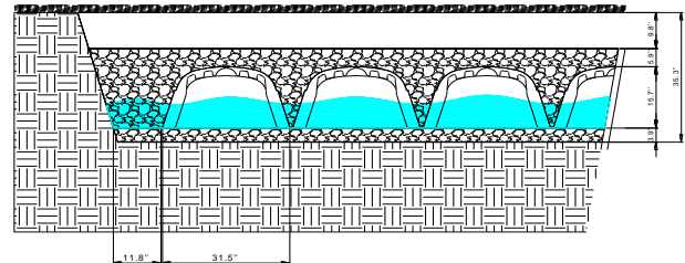
Fig. 1 – system cross-section
