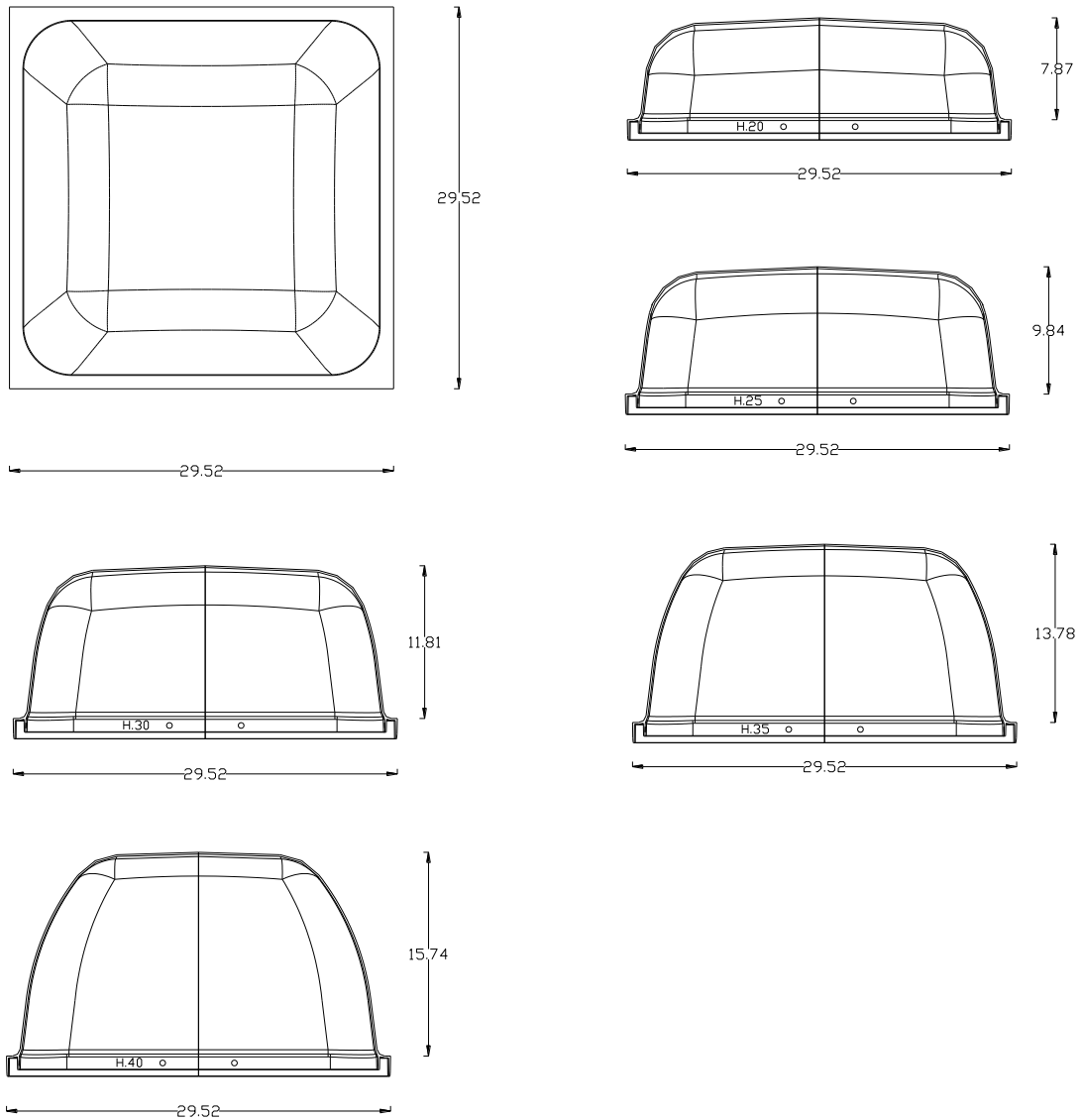
Plan view and cross-section of the Skydome forms [in]
