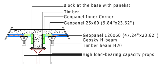
Solution for the closure of a slab with GEOPANEL outer corner and beams
